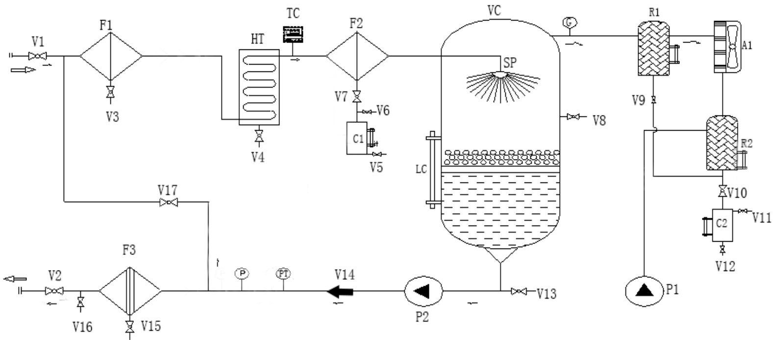
Flow Diagram For VHF Hydraulic Oil Purifier
